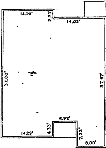
UNIT "A" 50 FT INTERIOR AIR SPACE 1040
